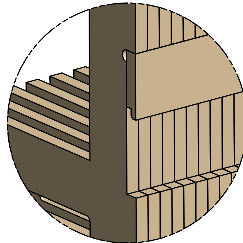
DETAIL J SCALE .35
