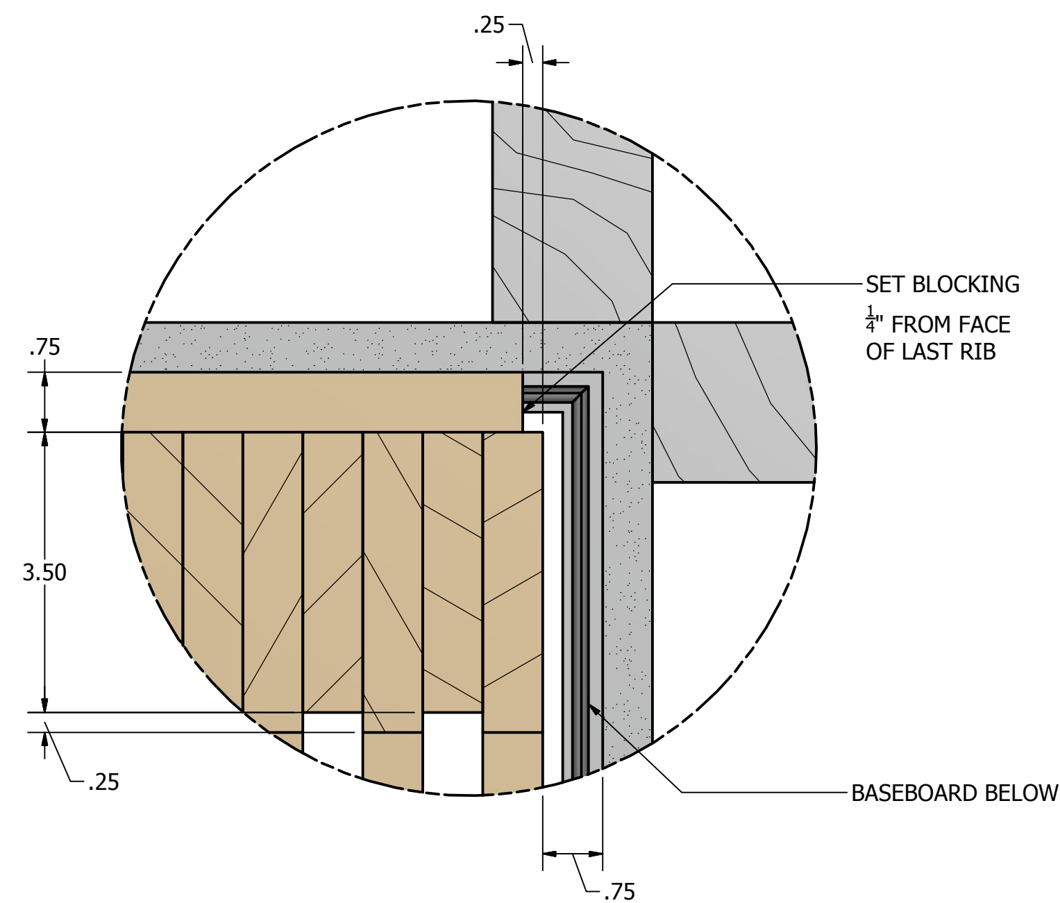
DETAIL F SCALE .6
