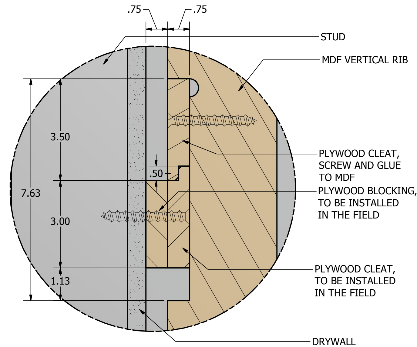
DETAIL C SCALE .5
