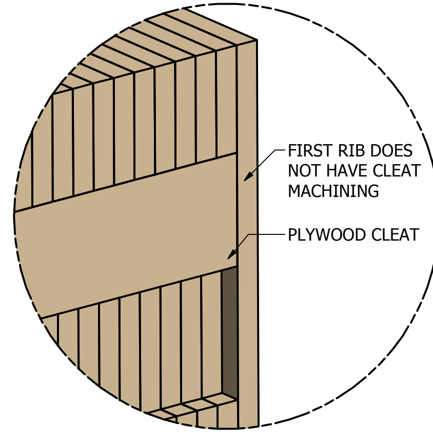
DETAIL H SCALE .35
