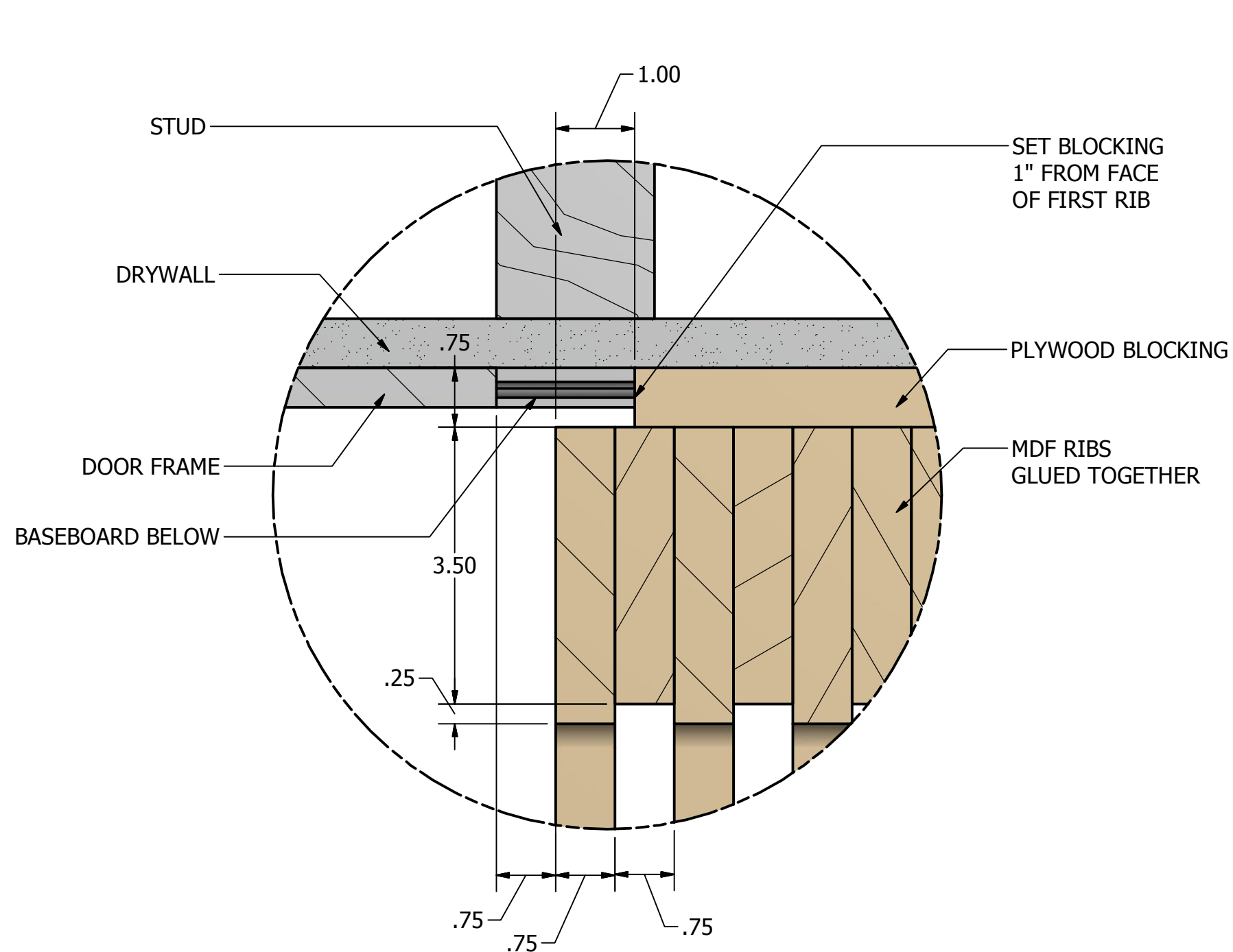
DETAIL G SCALE .6
