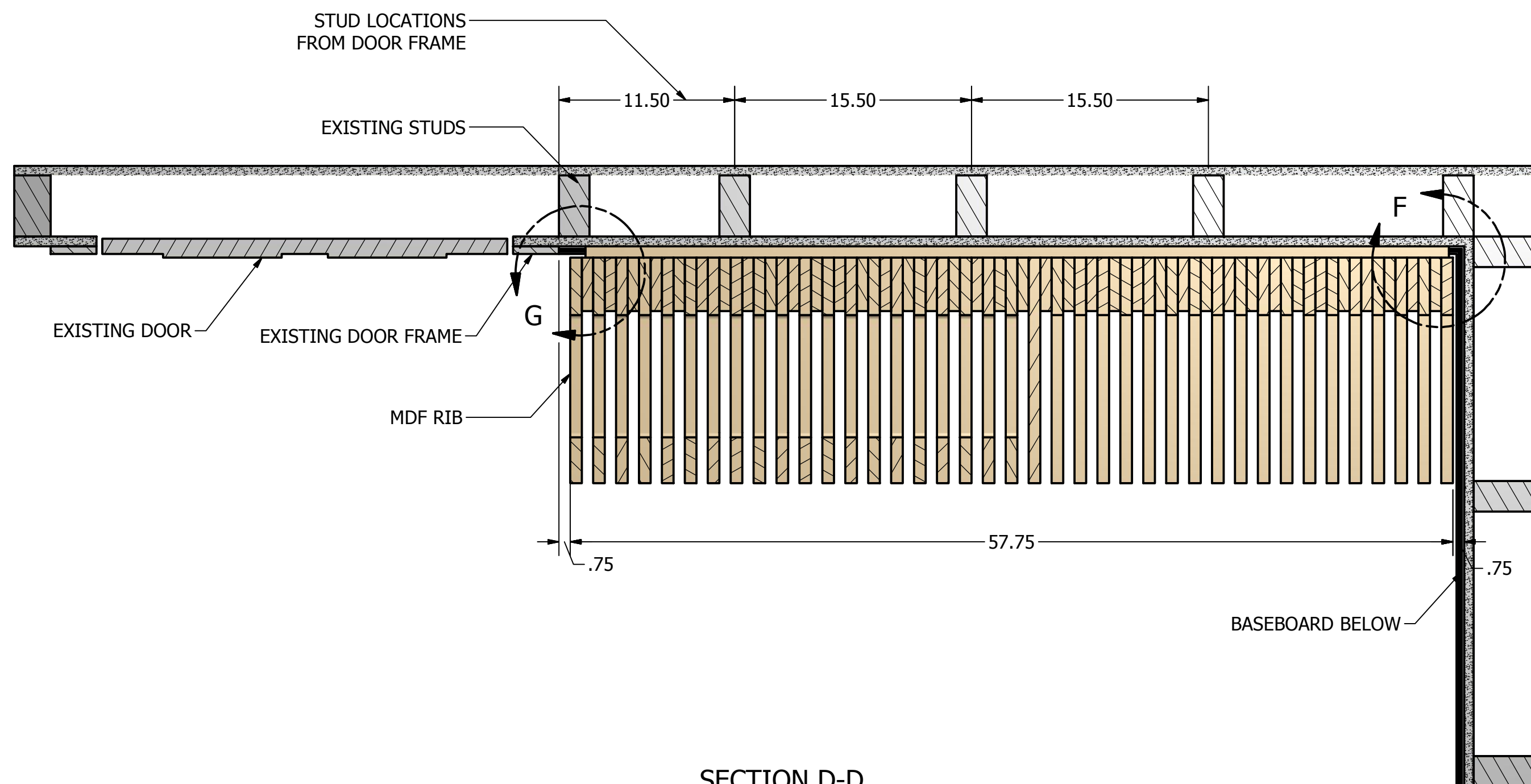
SECTION D-D SCALE .14
